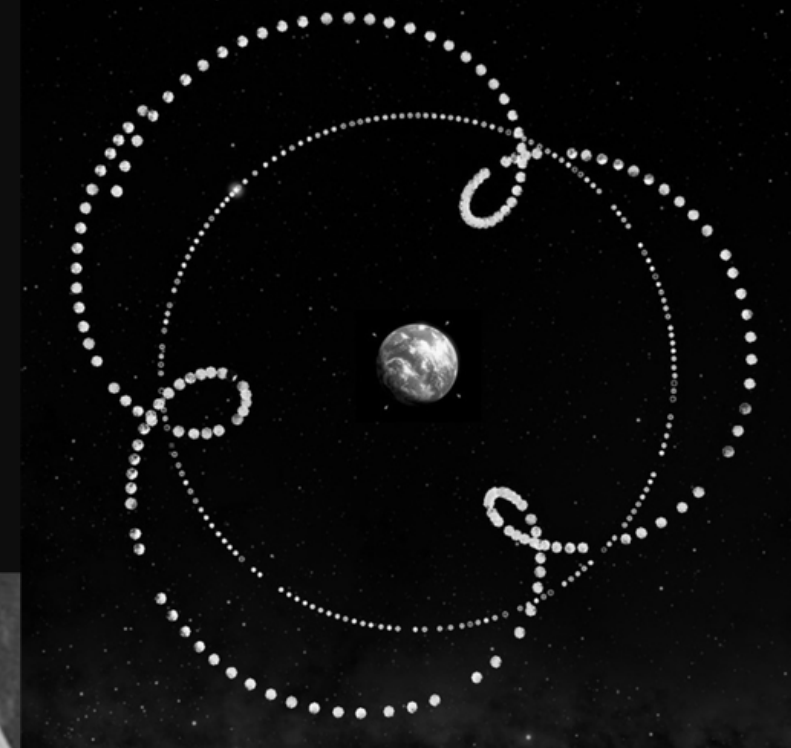
Mercury Pattern as Seen from Earth
