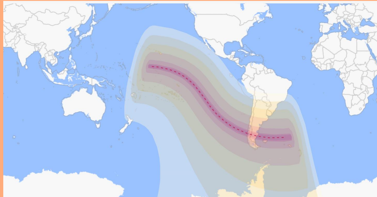
New Moon Annular Solar Eclipse
