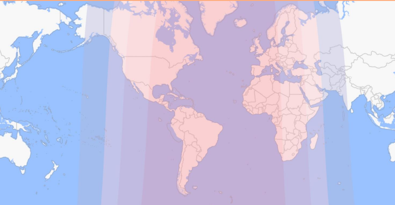
Full Moon Partial Lunar Eclipse
