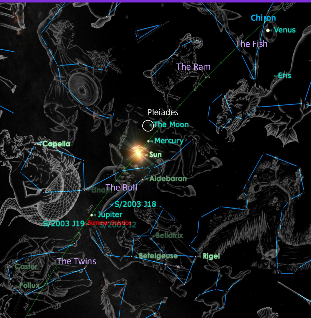
New Moon with Venus catching up to Chiron and Eris exact on June 1
